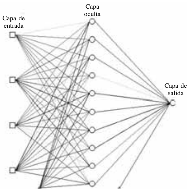
Figura 1. Red neuronal artificial. Artificial neural network.
