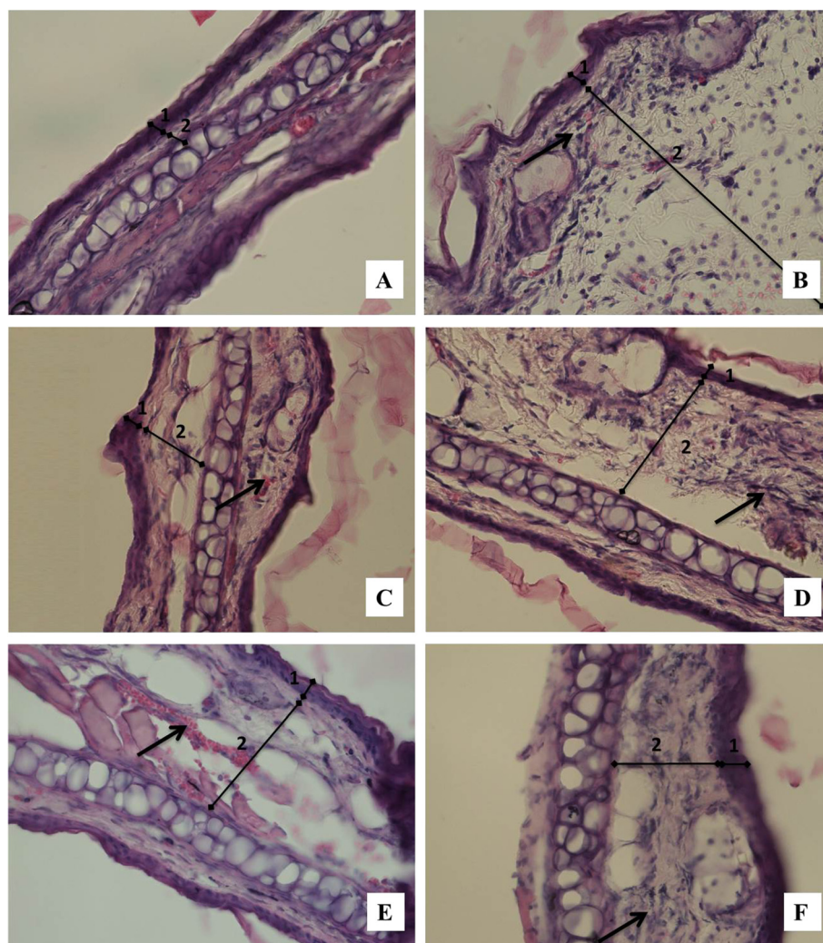
Figure 1 Histopathological changes produced by total extract and primary fractions of Cryptostegia grandiflora , qualified by a blinded pathologist. Pictures represent sections from mice ears stained with hematoxylin and eosin (40X) from: (A) Healthy group, (B) Control group (TPA, 2.5 µg/ear), (C) TPA and Indomethacin (0.5 mg/ear), (D) TPA and Cryptostegia grandiflora total extract (1.0 mg/ear), (E) TPA and Cryptostegia grandiflora ether fraction (1.0 mg/ear), and (F) TPA and Cryptostegia grandiflora dichloromethane fraction (1.0 mg/ear). The numbers 1 and 2 indicate epidermis and dermis, respectively. Arrows indicate cell infiltration into the dermis.
