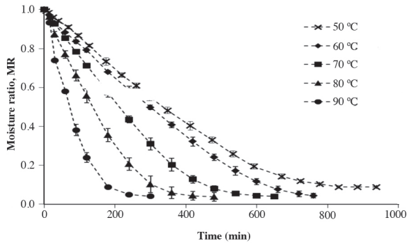
Figure 1. Experimental drying curves for goldenberry samples at different air-drying temperatures. Results are mean ± standard deviation, n = 3.
