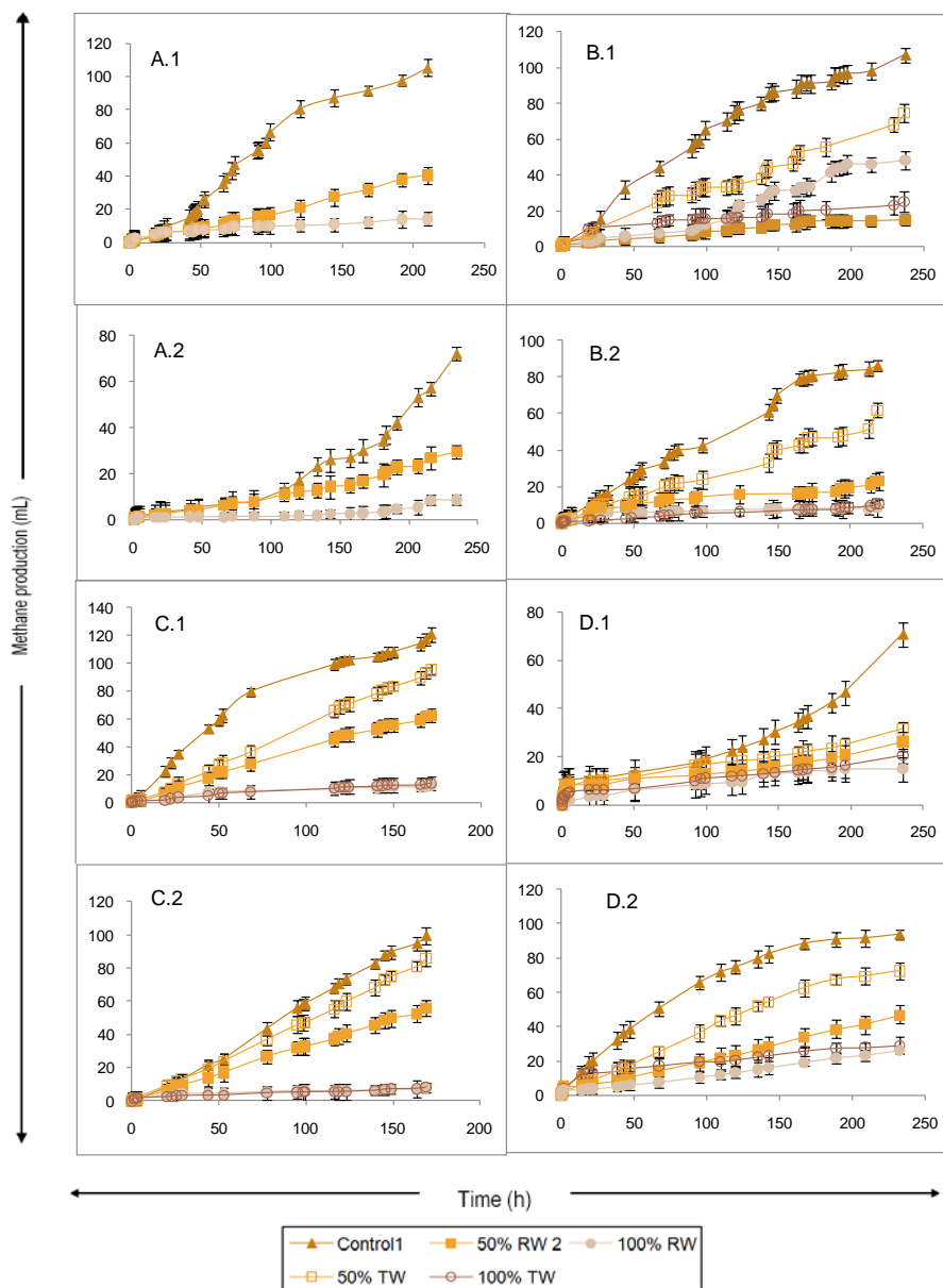
Fig. 1 Methane production in the methanogenic toxicity assays of piggery wastewater (1) first feeding and (2) second feeding. Assays corresponding to: A) serie A; B) serie B; C) serie C; and D) serie D.
