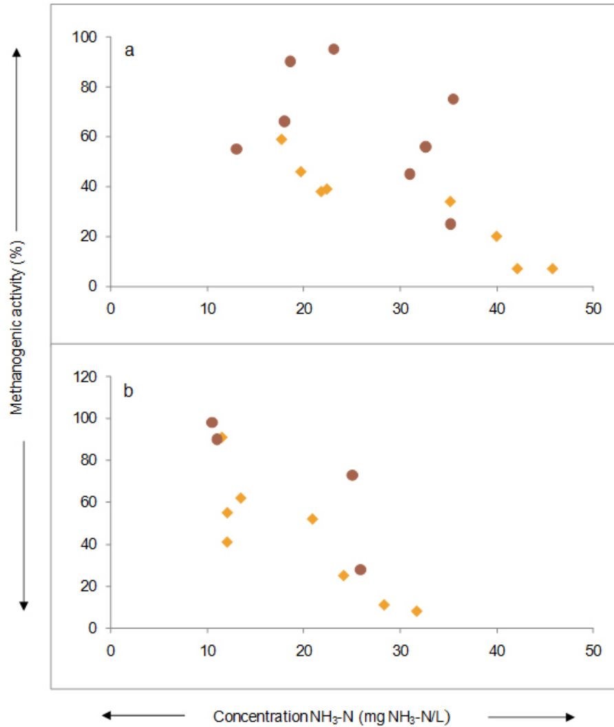
Fig. 2 Behavior methanogenic activity and free ammonia concentration for RW (a) and TW (b). Sludge flocculent (●) and granular (◆).
