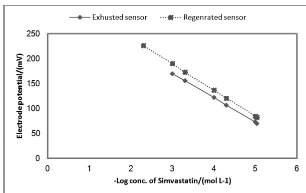
Figure 4: Regeneration of SIM-PMA Coated Wire Sensor.
