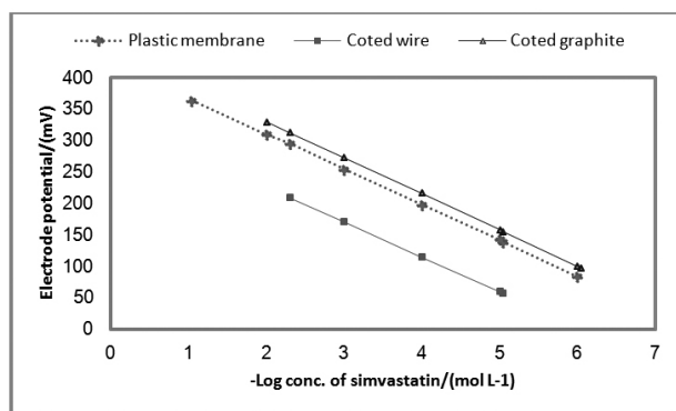
Figure 2: Typical Calibration Graphs of Simvastatin Sensors.
